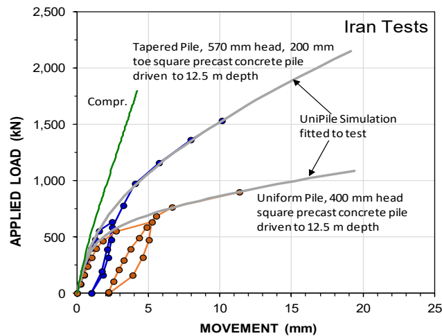
Figure 1. Comparison between 12.5 m long tapered and uniform square precast piles with UniPile simulations.
